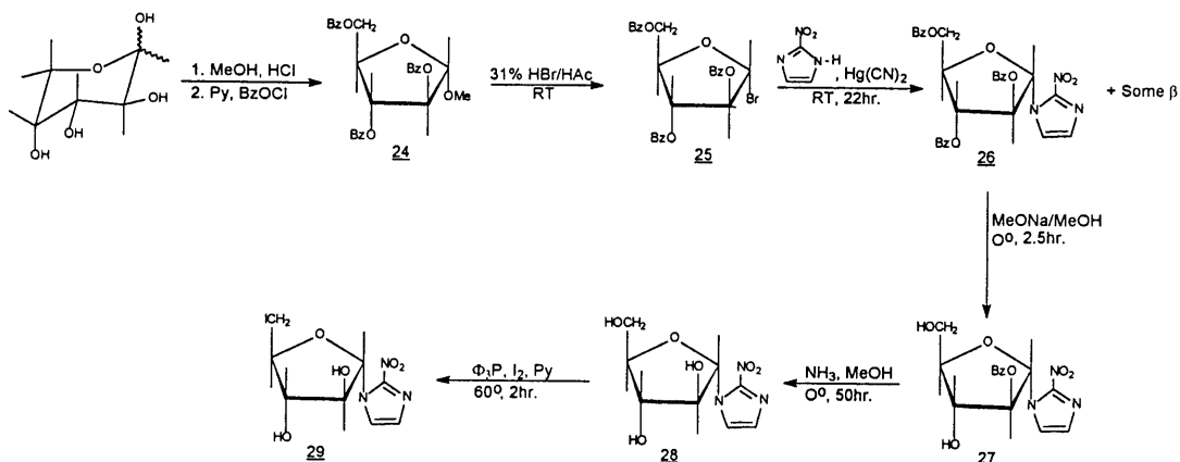
Figure 3: Synthesis of 29 .
